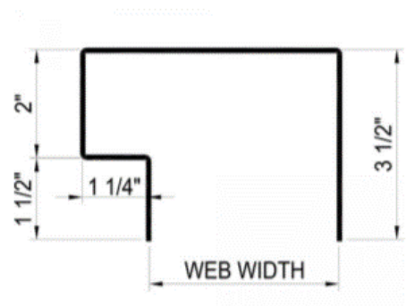
#14 2 HR, 2" total deflection
